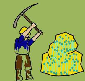
DATA MINING
