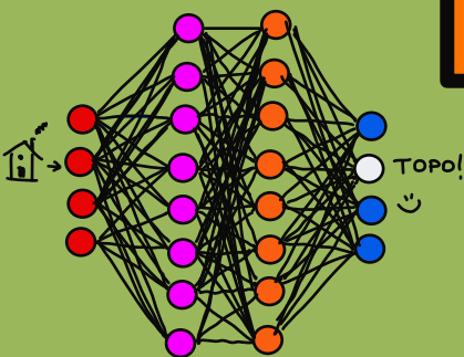
MACHINE LEARNING
