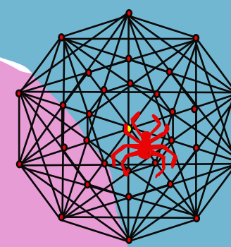
COMBINATORIA
