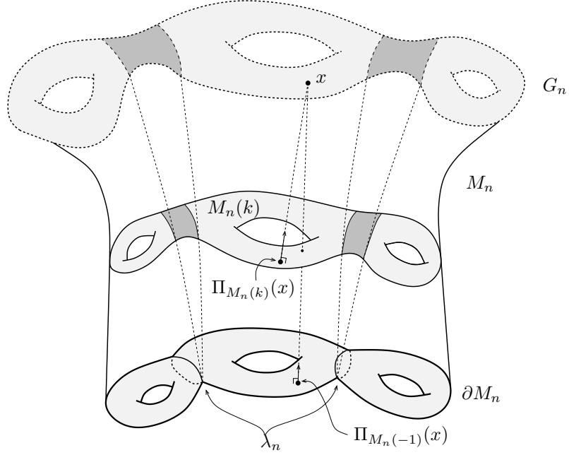
FIGURE 1. The retraction \Pi_{M_n(k)} .
