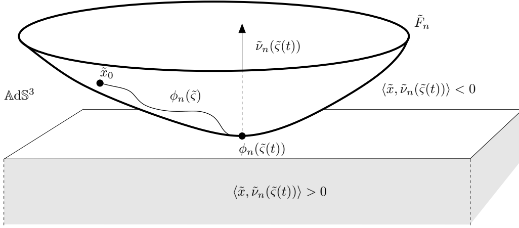
FIGURE 2. The product \langle \tilde{x}_0, \tilde{\nu}_n(\zeta(t)) \rangle is negative.
