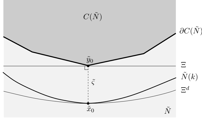
FIGURE 3. Estimating the distance between \tilde{N}(k) and C(\tilde{N}) .
