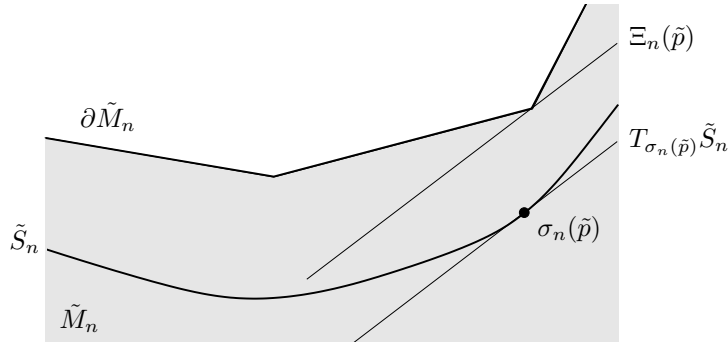
FIGURE 4. Convergence of the support planes.
