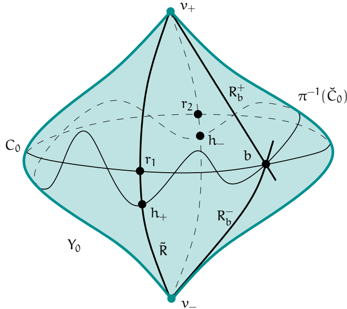
FIGURE 4. The double cover Y_0 of the quartic cone V_0 .
