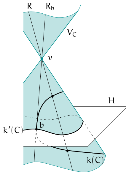
FIGURE 3. The quartic cone V_C for a hyperelliptic C .
