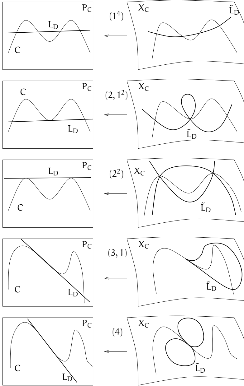
FIGURE 1. The non-hyperelliptic strata and the cover X_C \rightarrow P_C .
