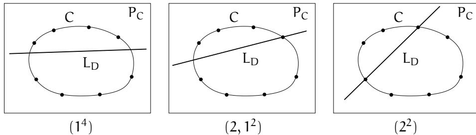
FIGURE 2. Hyperelliptic degenerations in the strata (1^4), (2, 1^2), (2^2) .
