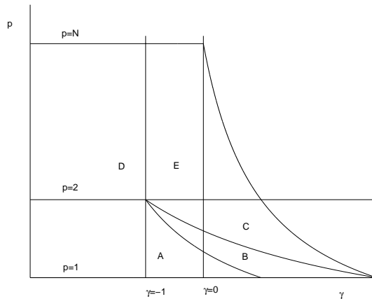
Figure 1: Summary of the existence and non-existence results for \lambda > \lambda_{N,p,\gamma} .
